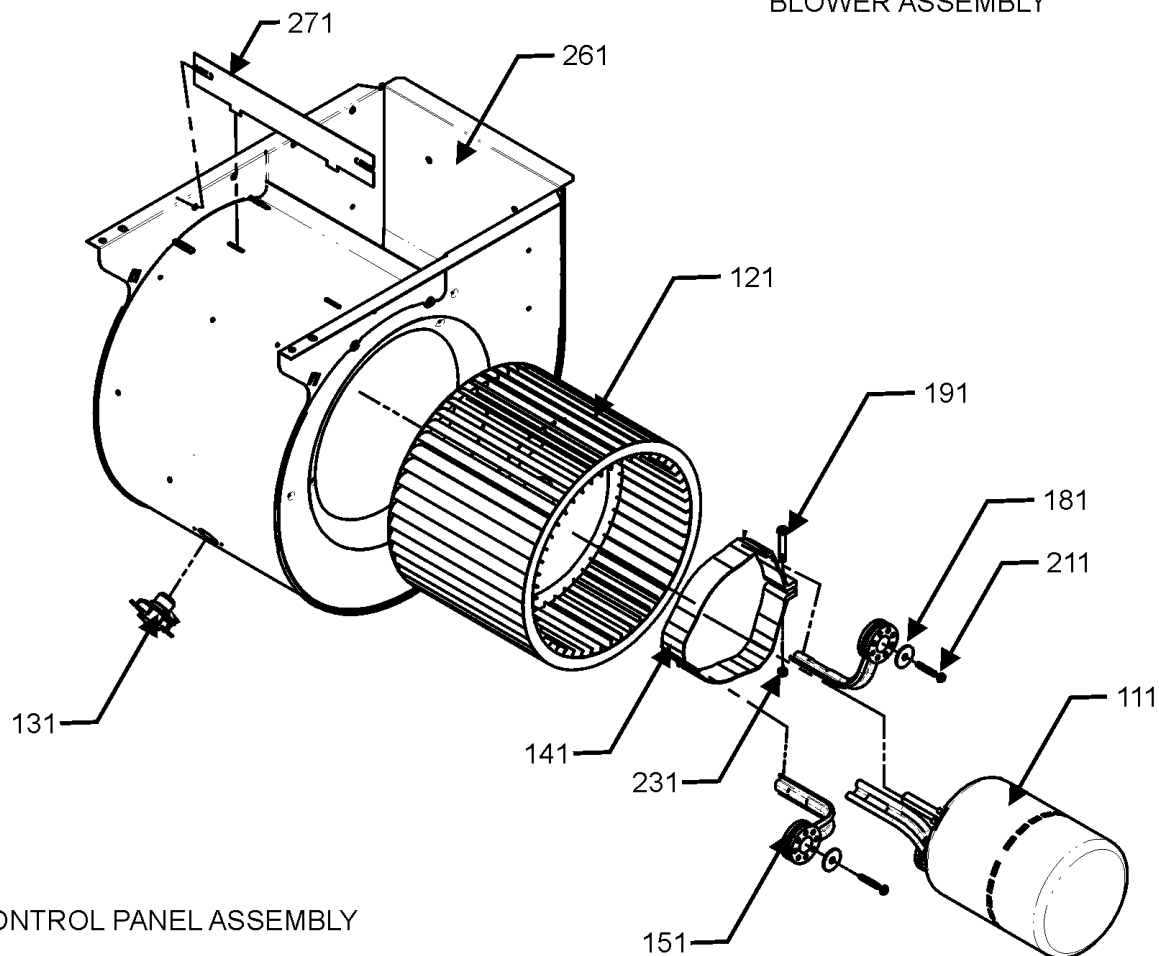
BLOWER ASSEMBLY
