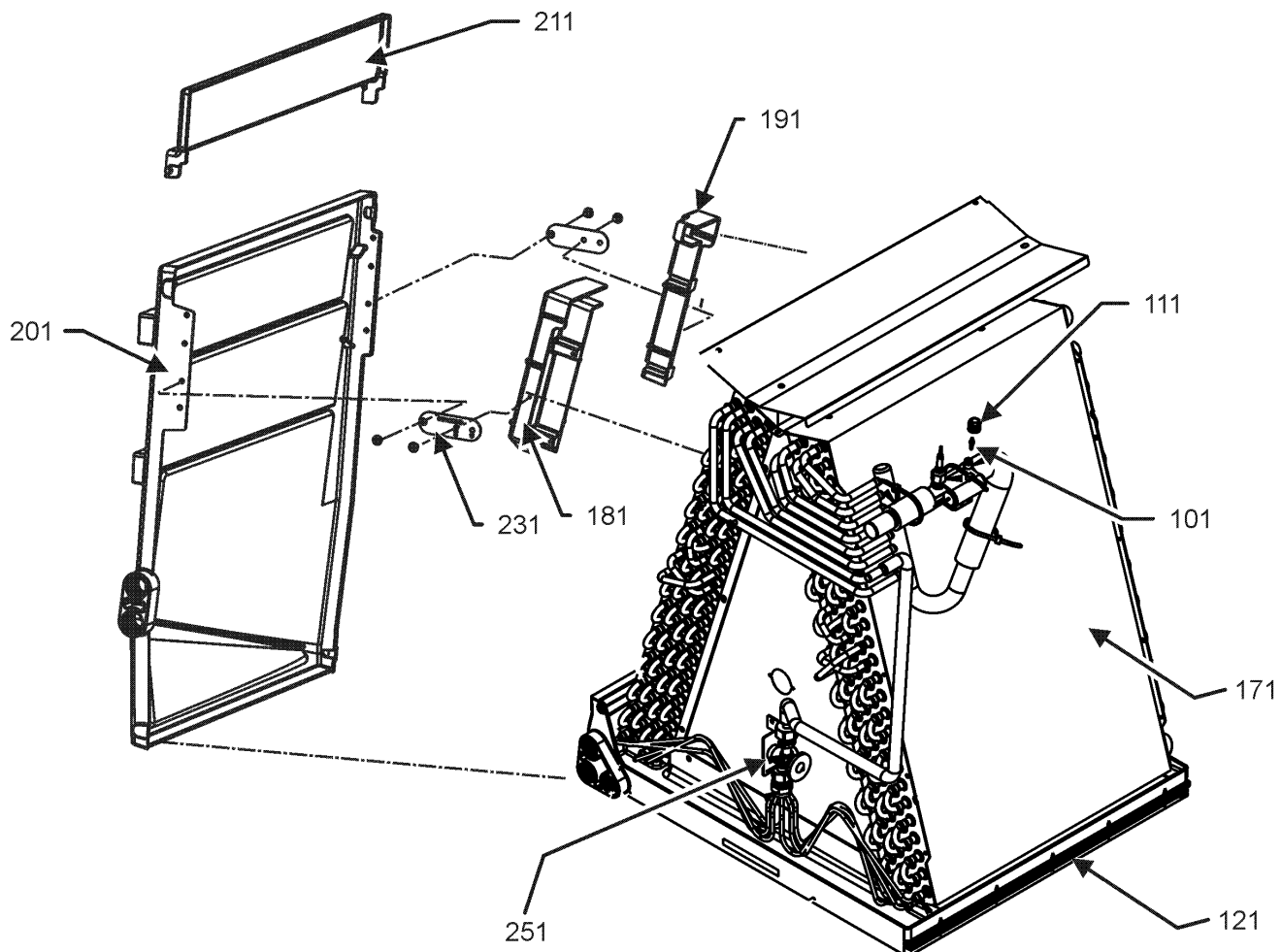
COIL TUBING ASSEMBLY
